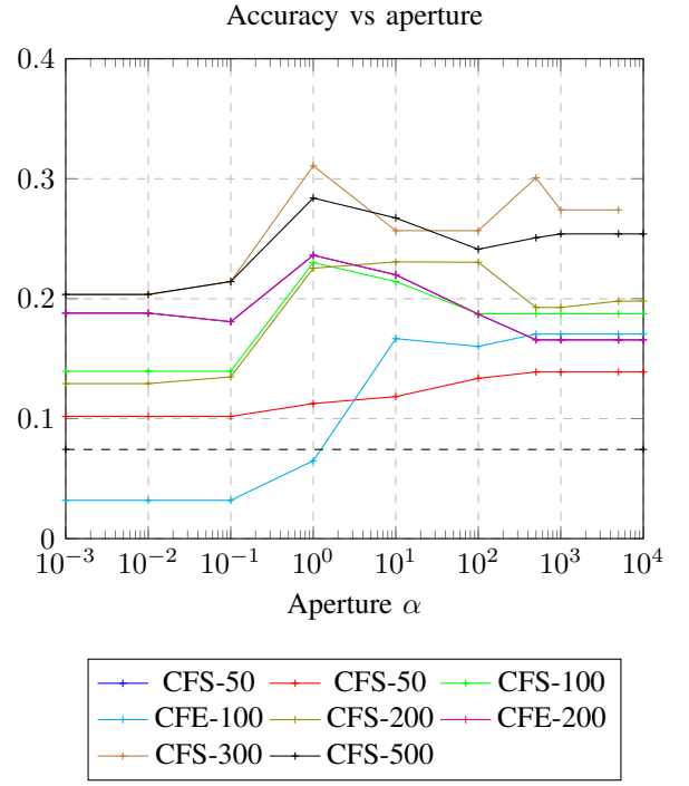
Fig. 1: 10-Fold cross-validation accuracy of ESN and Conceptors models on the HorseTrack dataset with various leaky rates, apertures and reservoir sizes.
