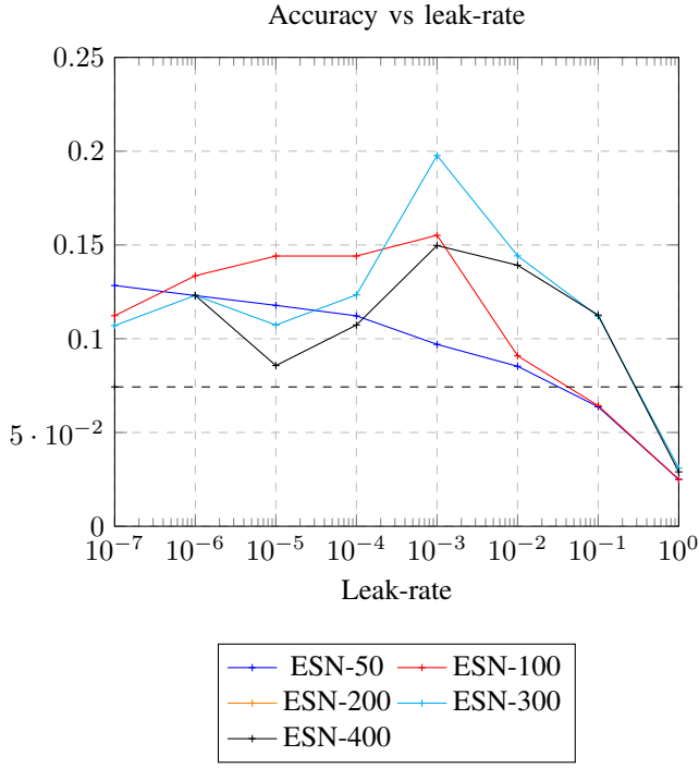
Fig. 1: 10-Fold cross-validation accuracy of ESN and Conceptors models on the HorseTrack dataset with various leaky rates, apertures and reservoir sizes.
